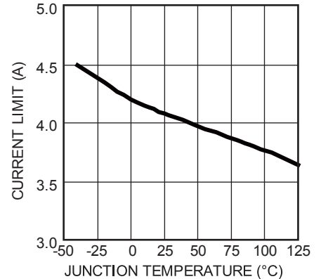
Current Limit vs. Junction Temperature Duty Cycle=40%
