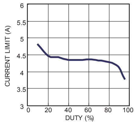
Current Limit vs. Duty T_J=+25^\circ C
