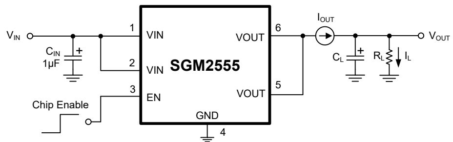
Test Circuit 2
