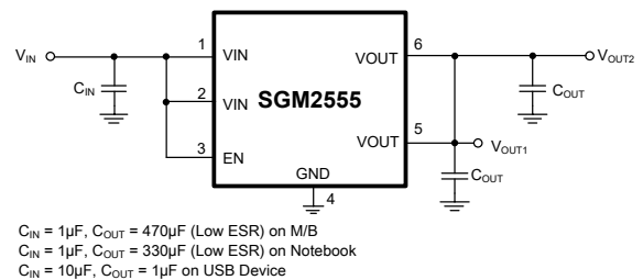
Figure 2. High-side Power Switch
