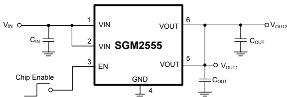
C IN = 1µF, C OUT = 470µF (Low ESR) on M/B C IN = 1µF, C OUT = 330µF (Low ESR) on Notebook C IN = 10µF, C OUT = 1µF on USB Device
