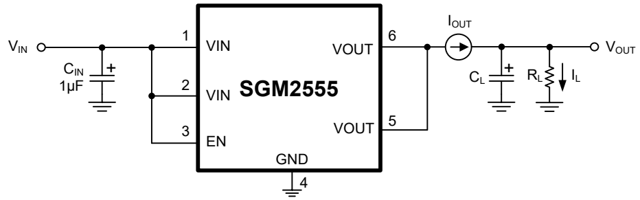
Test Circuit 1
